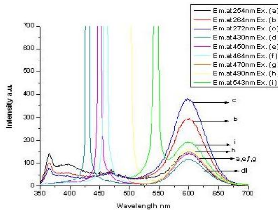
Fig. 2 : Emission spectra of SrS : Eu at different Excitations
