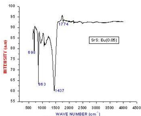
Fig. 2.12 FTIR of SrS:Eu(0.05)
